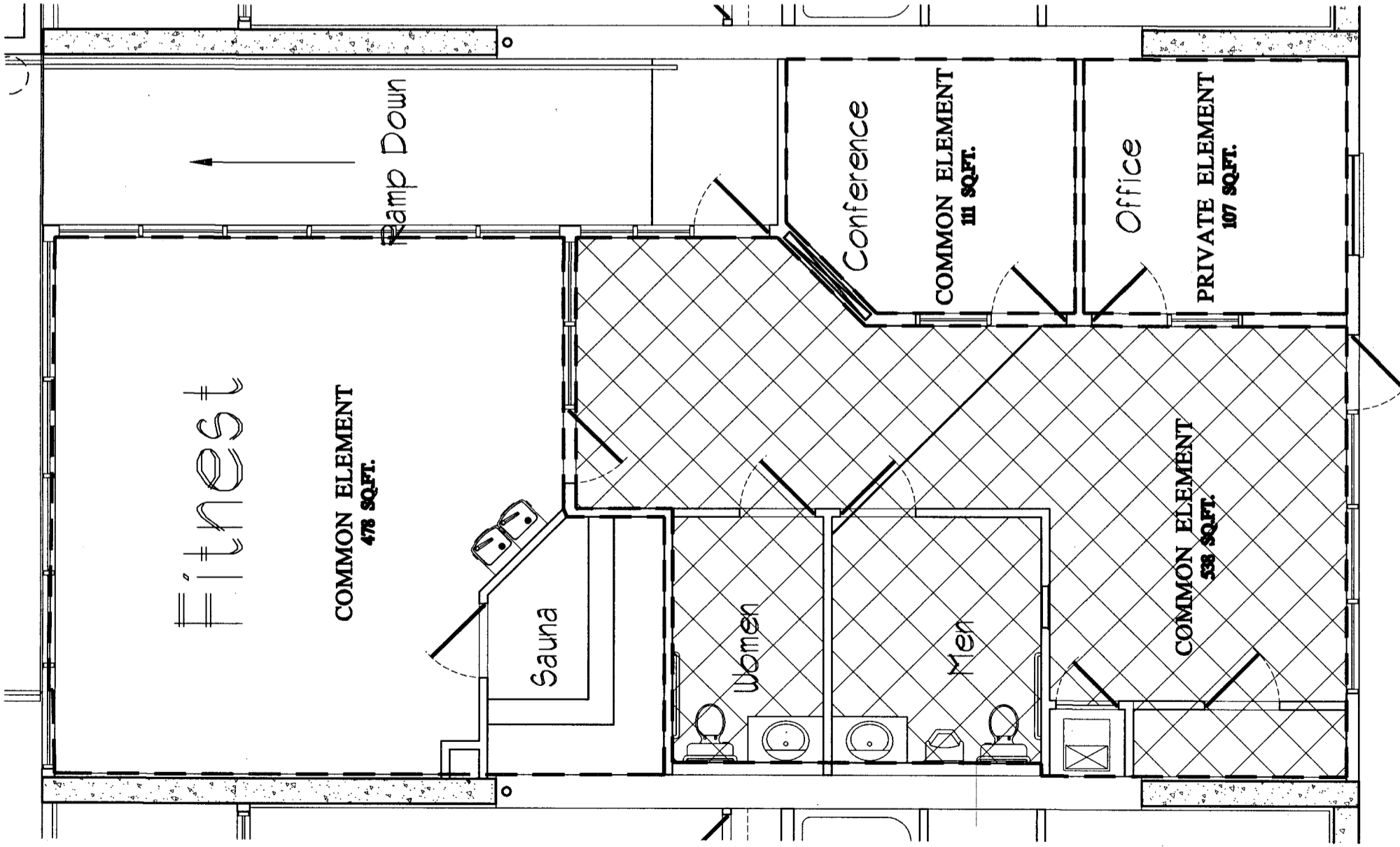
Common Lobby/Fitness Level 02 N.T.S.
