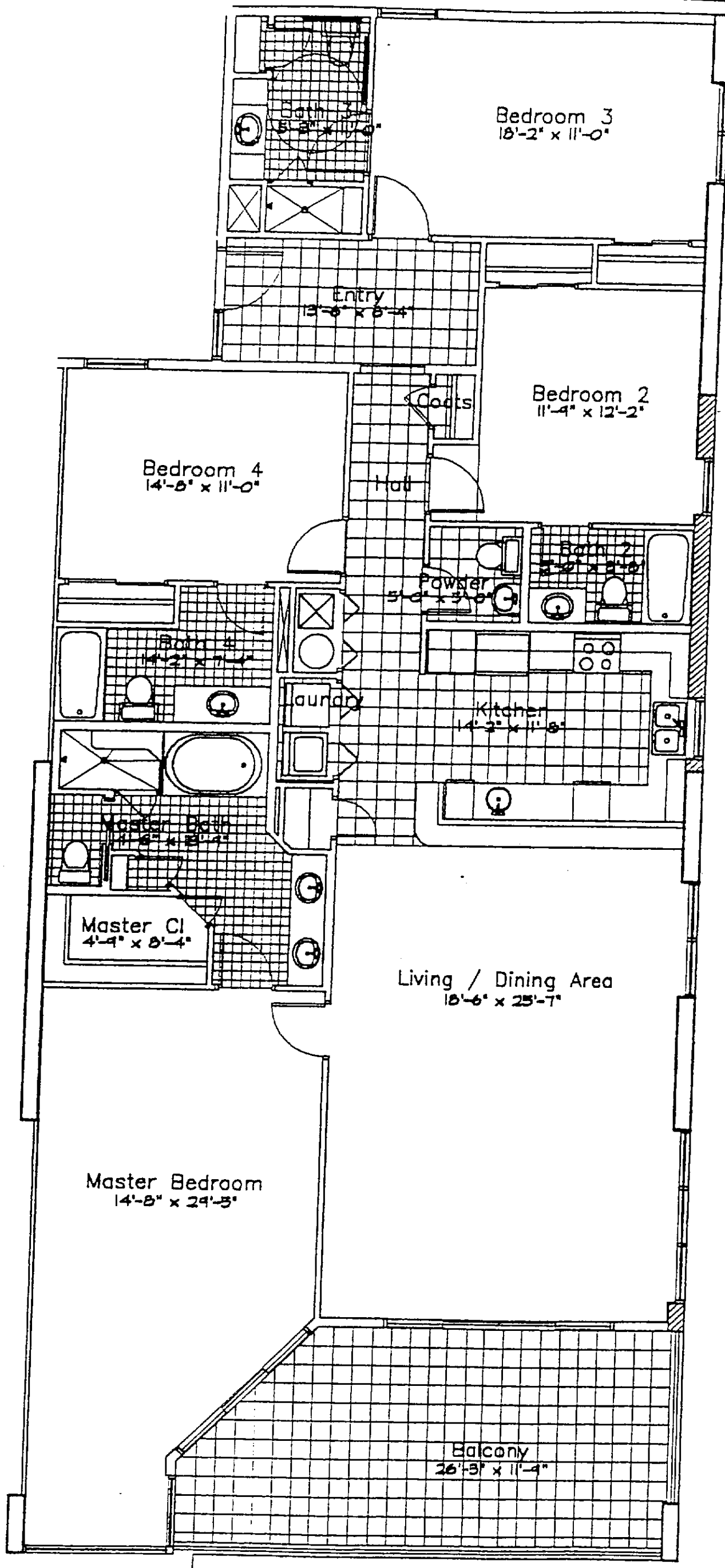
Unit "A" Plan - 4 Bedroom
