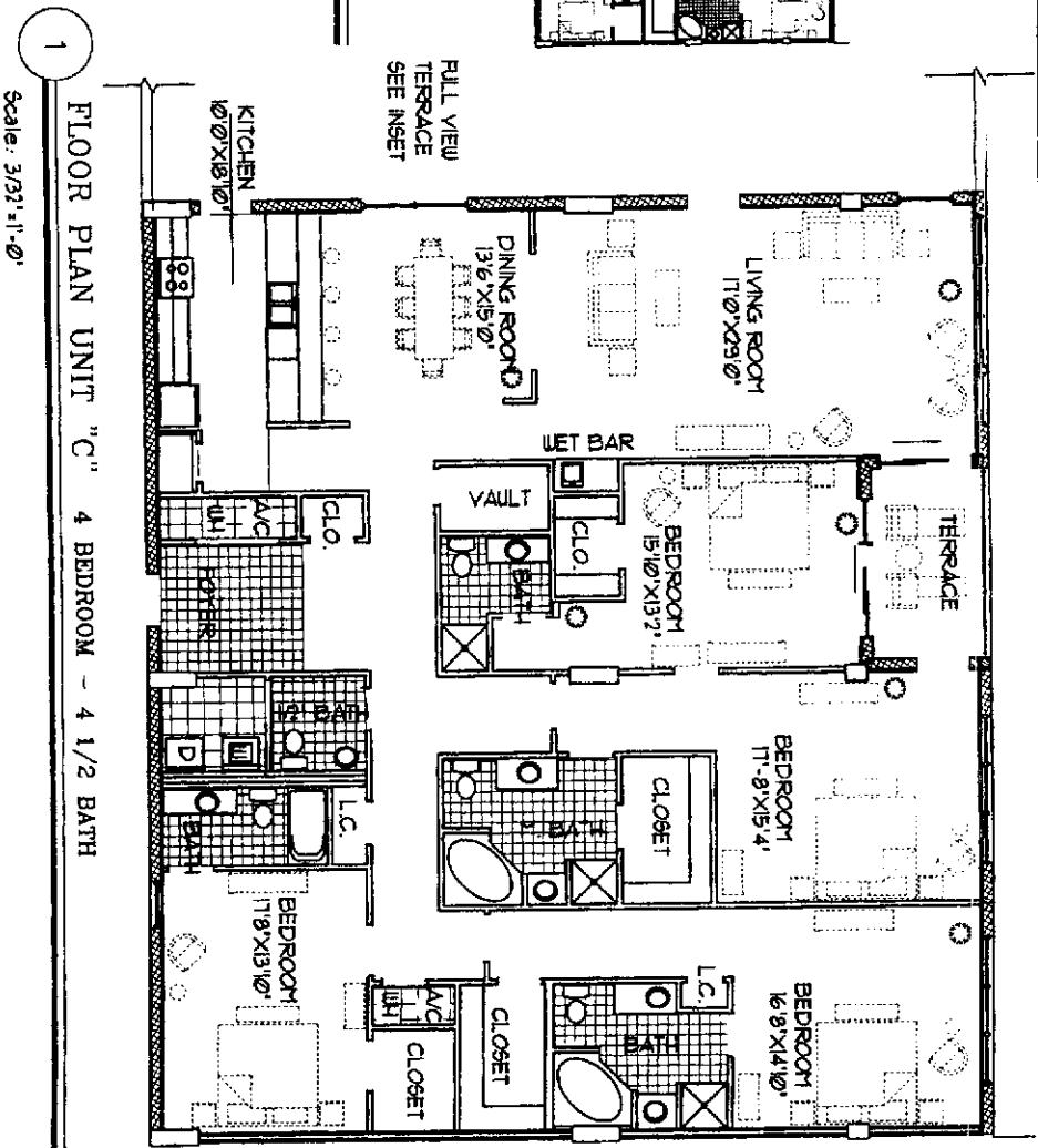
UNIT "C" INCLUDING TERRACE Scale: 1"=30'-0"
